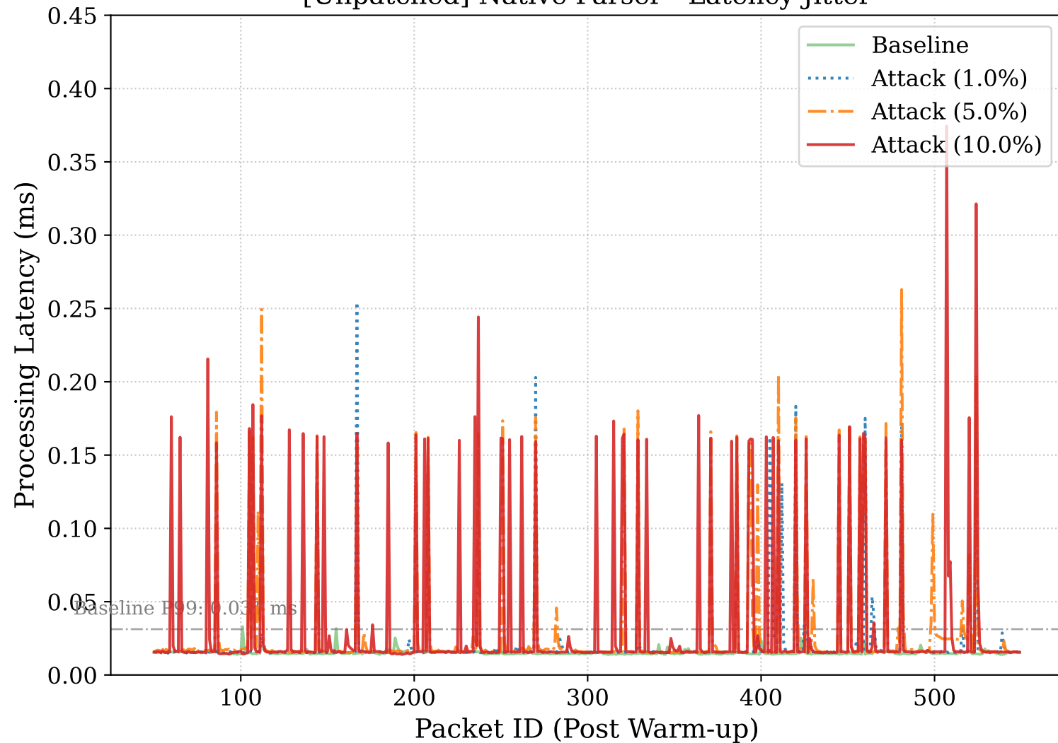
[Unpatched] Native Parser - Latency Jitter
