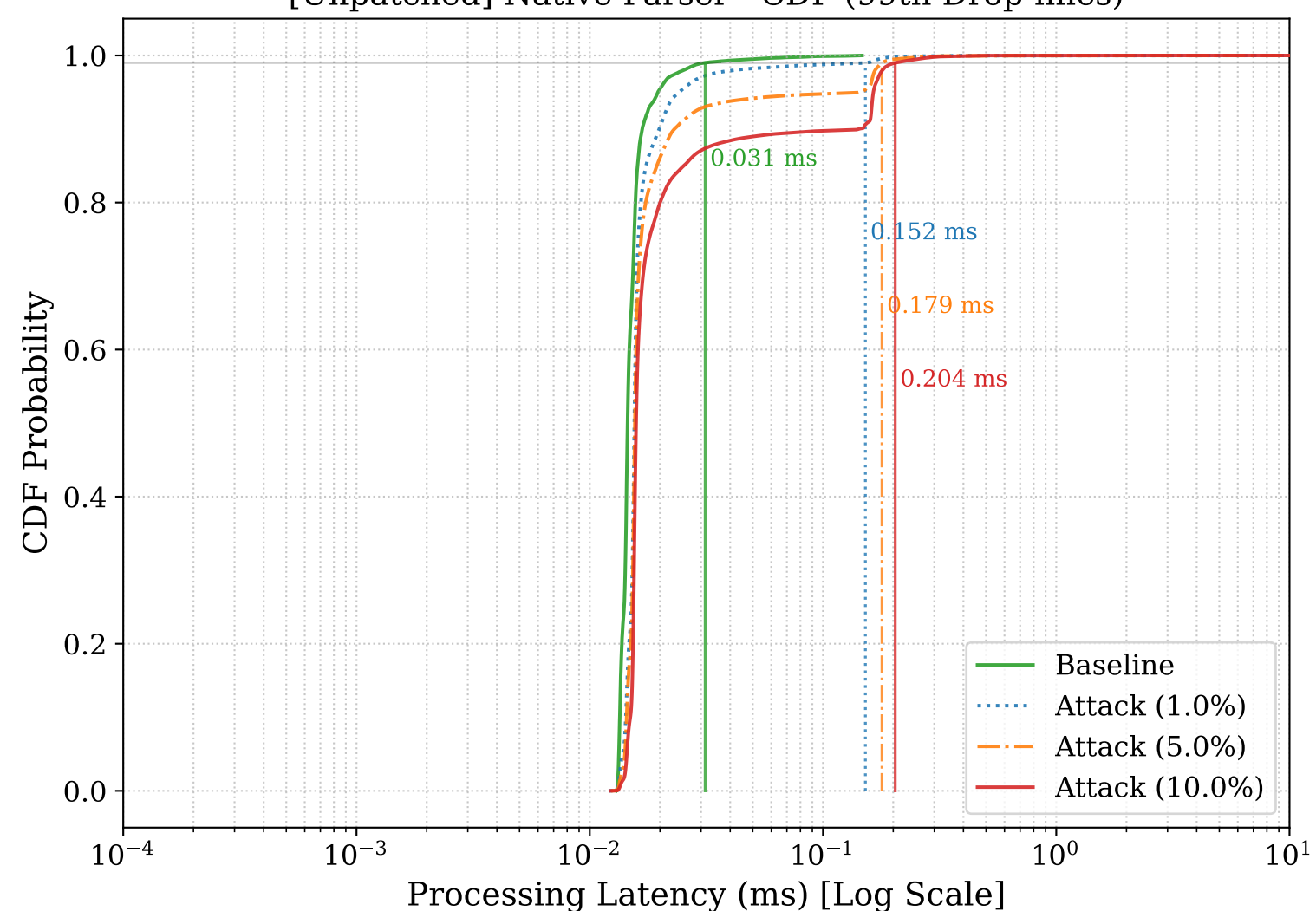
[Unpatched] Native Parser - CDF (99th Drop-lines)
